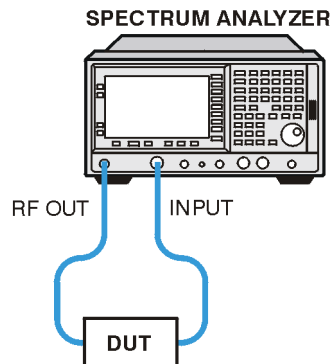
Figure 2-8 Transmission Measurement Test Setup
